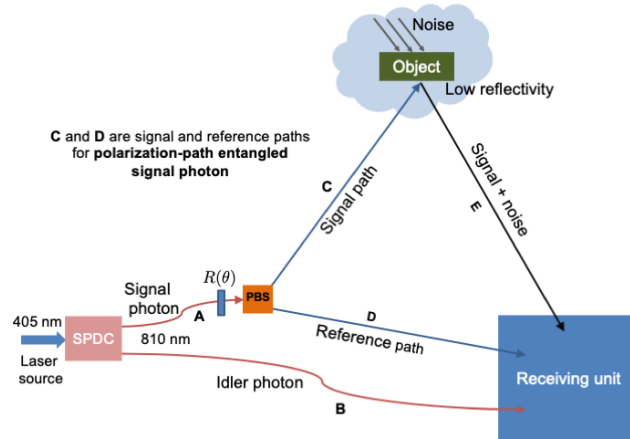
Fig. 1. Schematic of the quantum illumination protocol using polarization-path entangled single photons. Spontaneous parametric down conversion process is used to generate photons pairs and one of them, signal photon along path A is entangled in polarization and path degree of freedom and sent along signal path, C and reference path, D. Another photon from the pair along path B is used as idler for heralding signal photons. An object of different reflectivity is placed in the signal path with variable background noise. Entanglement between polarization and path degree of freedom using coincidence counts of photons along paths D and E is calculated with photons along B. Bell's inequality violation in the form of CHSH parameter S is used to quantify quantum correlation and object detection.
