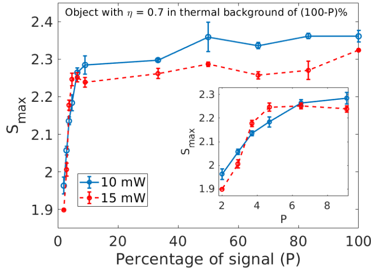
Fig. 5. Experimentally obtained maximum value of CHSH parameter S_{\max} for different percentage of signal ( P ) in presence of an object of reflectivity \eta = 0.7 . The background noise is increased such that the percentage of signal varied from 100 to 2. The solid and dashed line data points are for a pump power of 10 and 15 mW, respectively. The error bars are for the standard deviation of the measurements. The inset shows the zoomed region of the percentage of signal from 9 to 2. We can see that S_{\max} > 2 even when \text{SNR} = 0.03 .
